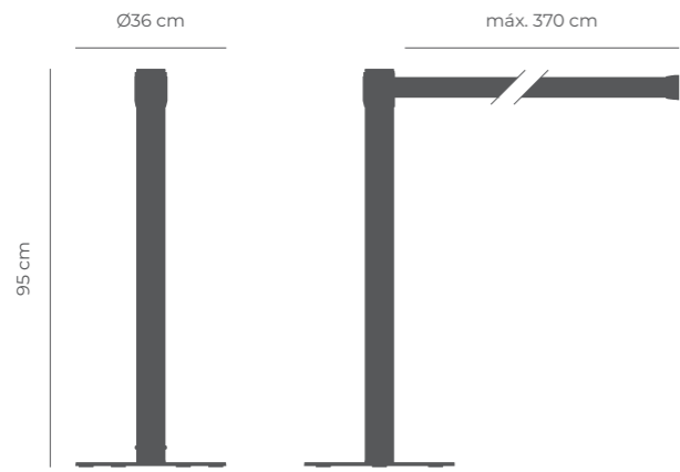
ECO post Esc. 1:20 (Weight: 8kg)
