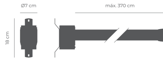
Vertical BASIC wall Esc. 1:10 (Weight: 1Kg)
