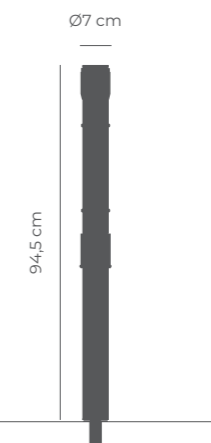
UNFIX DUAL post Esc. 1:20 (Weight: 4Kg)
