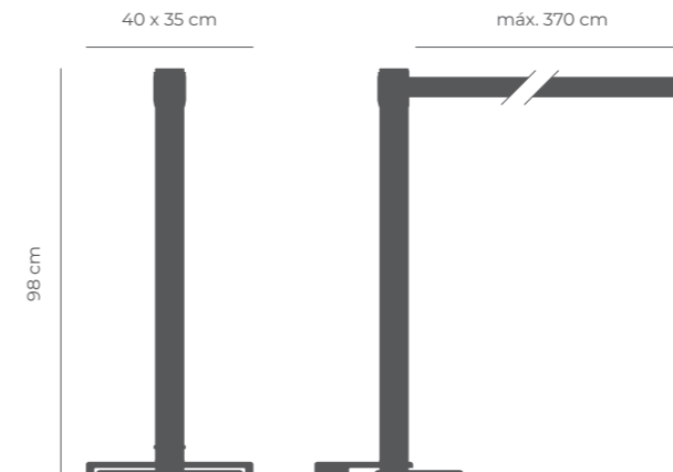
MAX post Esc. 1:20 (Weight: 11kg)
