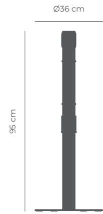
LIMIT DUAL post Esc. 1:20 (Weight: 11Kg)
