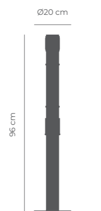
MAG DUAL post Esc. 1:20 (Weight: 4Kg)
