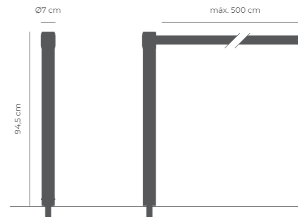
UNFIX post Esc. 1:20 (Weight: 4kg)
