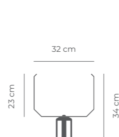
Notice holder ECO A4 H Esc. 1:20 (Weight: 0,7kg)
