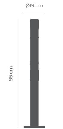
FIX DUAL post Esc. 1:20 (Weight: 4Kg)
