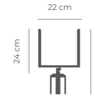
Notice holder BASIC A4 V Esc. 1:20 (Weight: 0,7kg)
