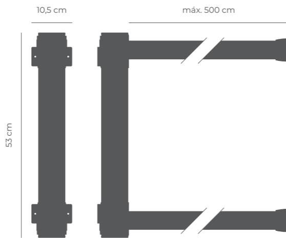
DUAL wall Esc. 1:10 (Weight: 2Kg)
