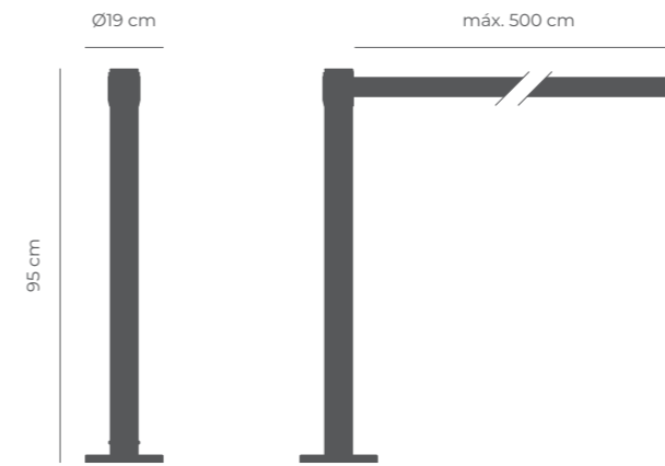
FIX post Esc. 1:20 (Weight: 4kg)
