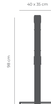
MAX DUAL post Esc. 1:20 (Weight: 11Kg)
