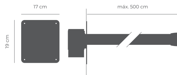
FIX wall Esc. 1:10 (Weight: 1kg)
