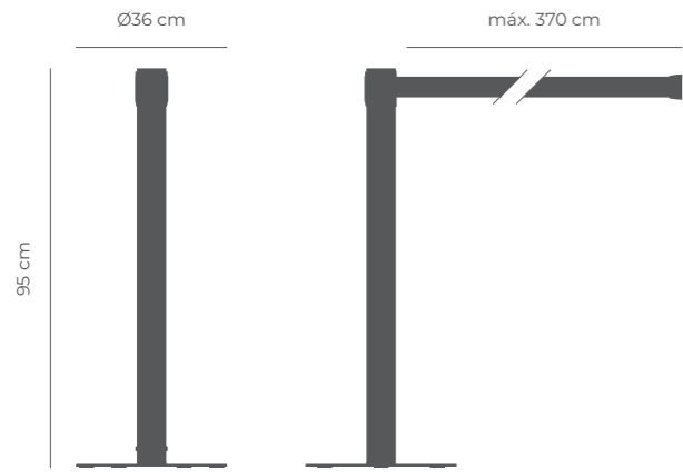
LIMIT post Esc. 1:20 (Weight: 11kg)
