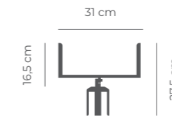
Notice holder BASIC A4 H Esc. 1:20 (Weight: 0,7kg)
